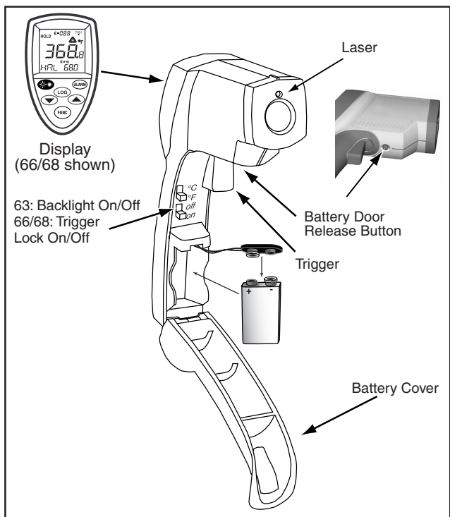
Figure 2. Infrared Thermometer
