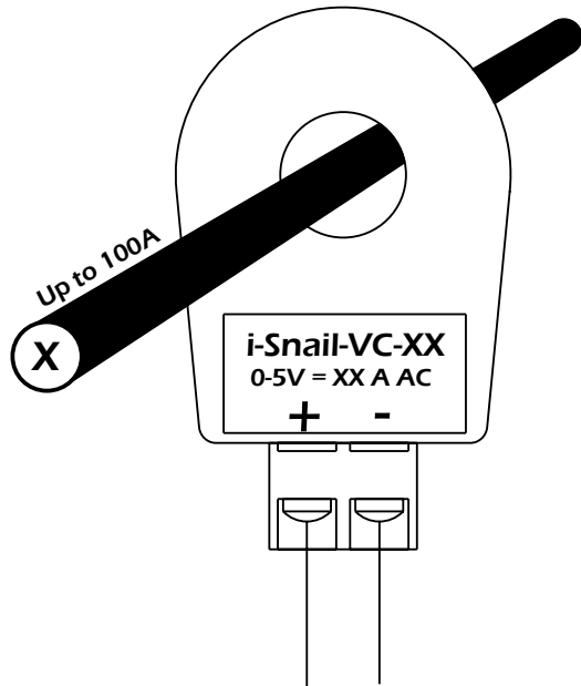
Linear 0-5Vdc representing 0-XX Amps
